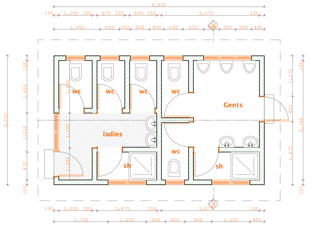
Floor plan
